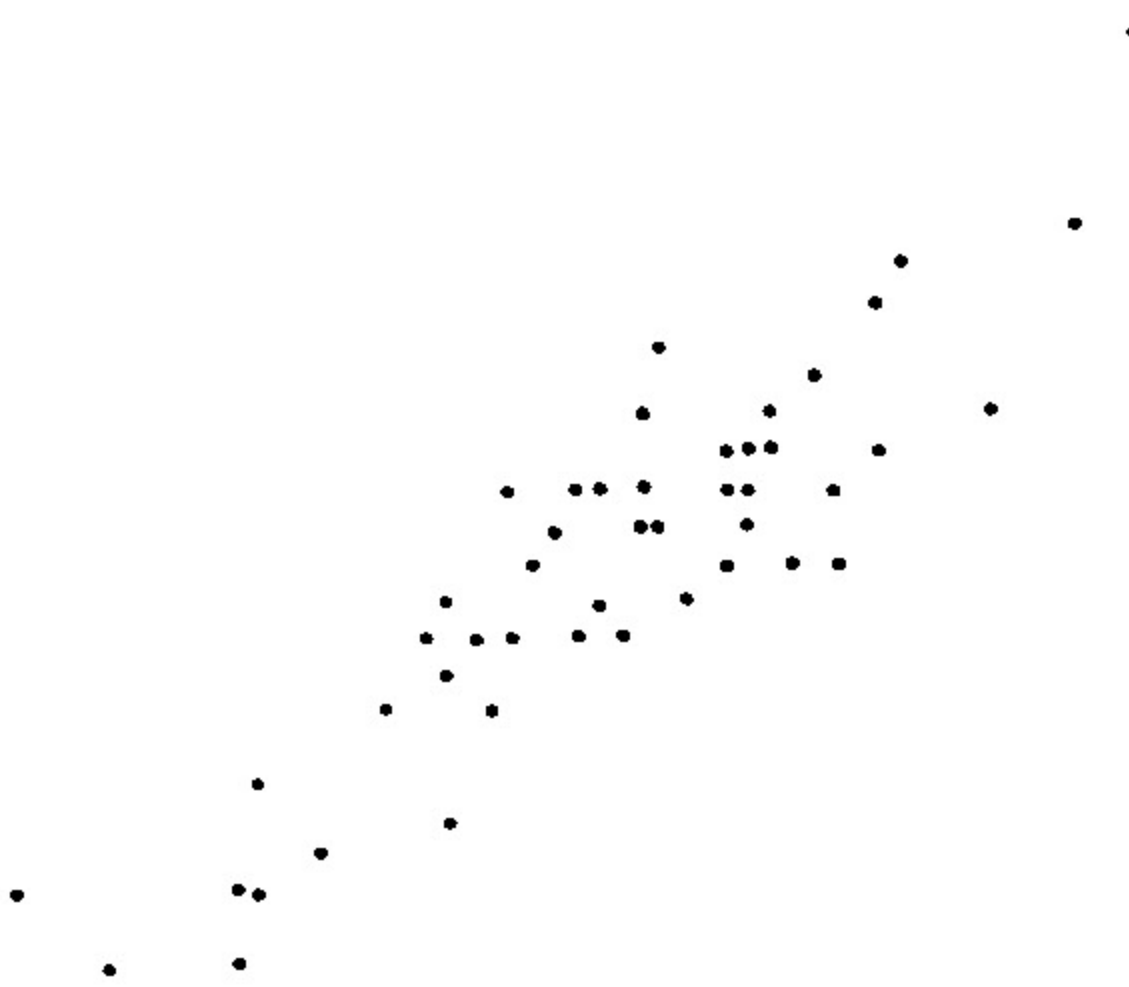
(e) Correlation r = 0.91
